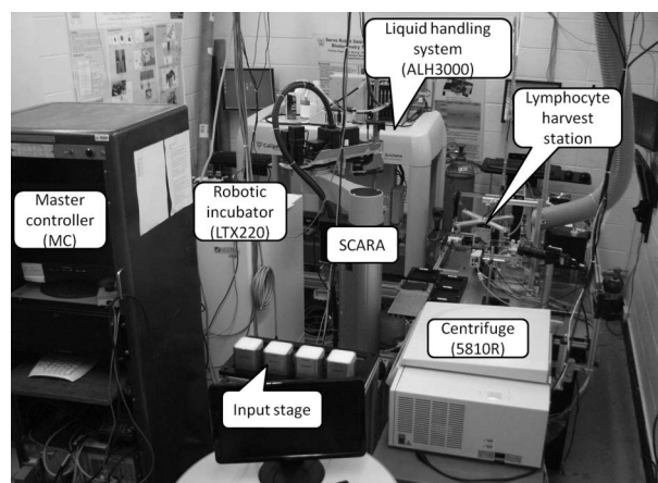
Figure 2. Photo of the RABiT, showing the various subsystems. The Lymphocyte Harvest station is shown in close up in Figure 5. The imaging system is shown in Figure 8. The transfer to substrate system is described in Chen et al. (2010b).
