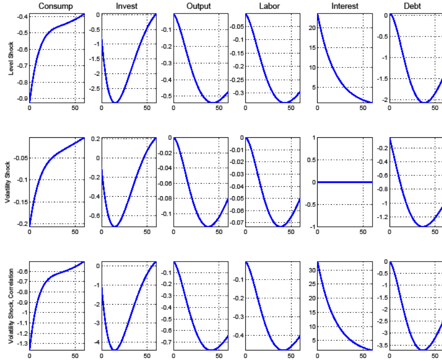
Figure 8: IRFs Ecuador
