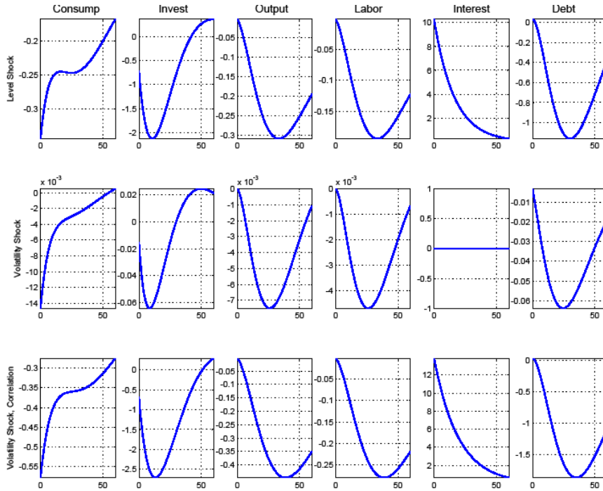
Figure 9: IRFs Venezuela
