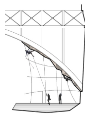
1 | OVERHEAD CLIMBING HEIGHT: 30' EAST STREET ARCHWAY
