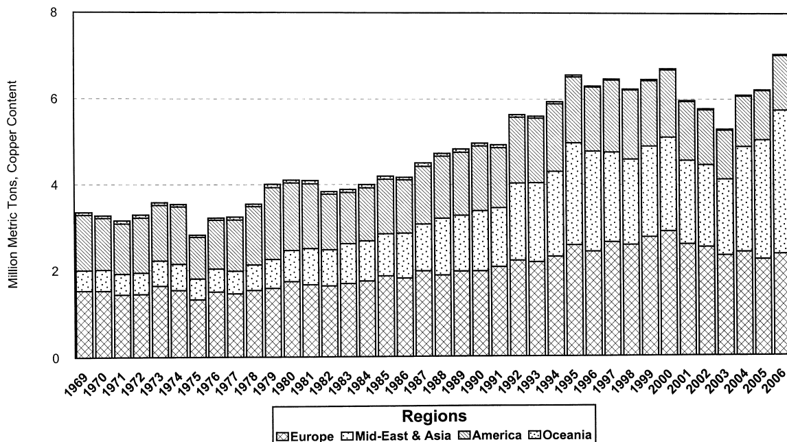
Figure 3. World Consumption of Copper of Direct Melt and Refined Scrap, by Region, 1969–2006
