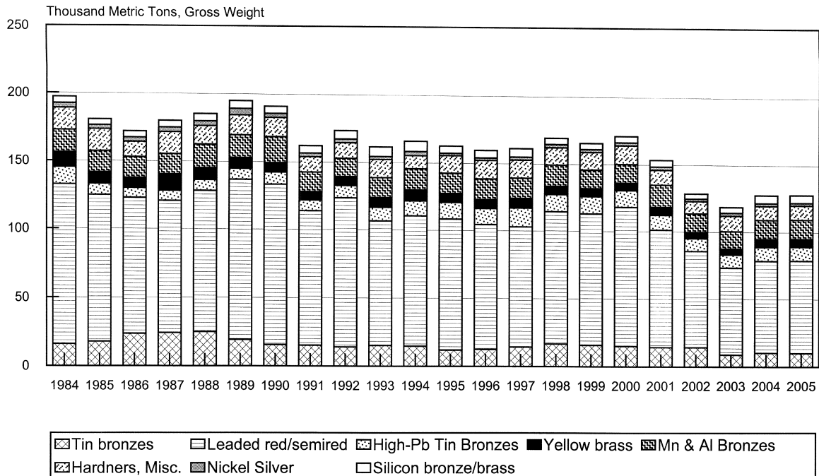
Figure 7. U.S. Copper Alloy Ingot Production by Ingot Group, 1984–2005
