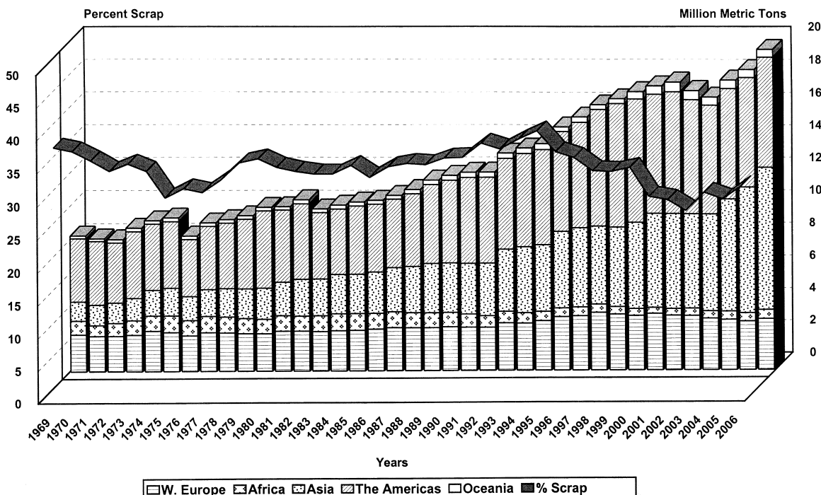
Figure 2. World Copper Recovery from All Sources 1 and Percent Copper from Scrap, 1969–2006
