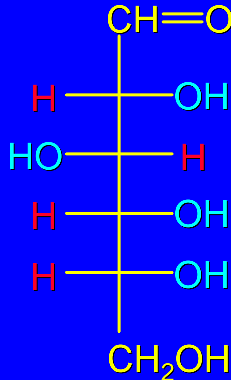
D-(+)-Glucose
