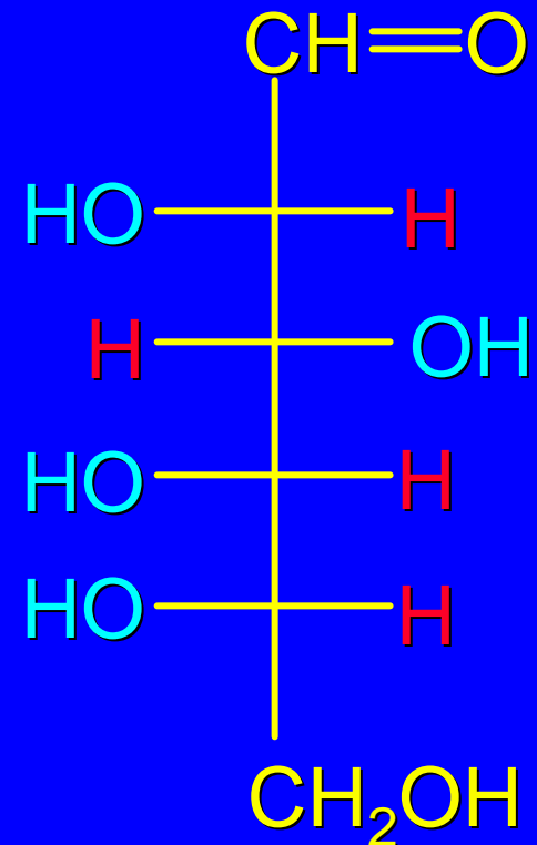
L-(−)-Glucose
