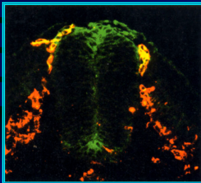
HNK-1 = crest
